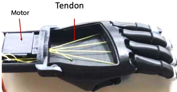
Figure 10. Overall assembly of the prototype
