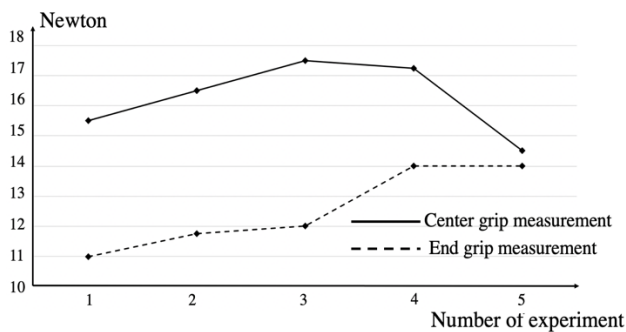
Figure 14. Squeezing force between center squeezing measurement and end squeezing measurement
