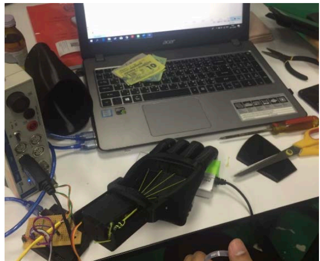
Figure 12. Center squeezing measurement
