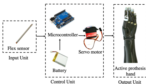
Figure 1. Diagram of active prosthetic hand prototype
